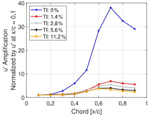
(b) Amplification of streamwise velocity fluctuations.
