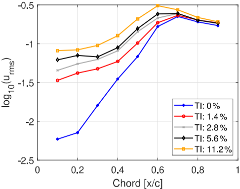
(a) Development of streamwise velocity fluctuations.
