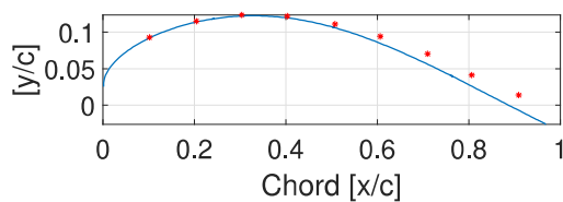
(f) Data output locations at the height of displacement thickness (shown here: case without added inflow turbulence).
