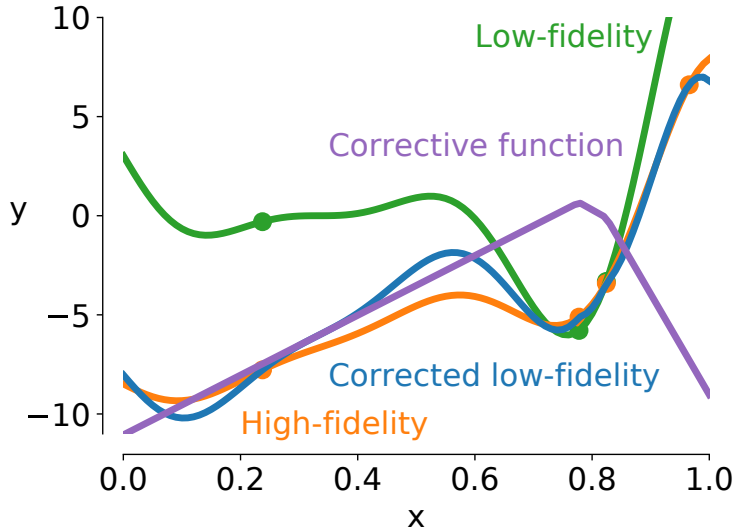
(a) Piecewise-linear
