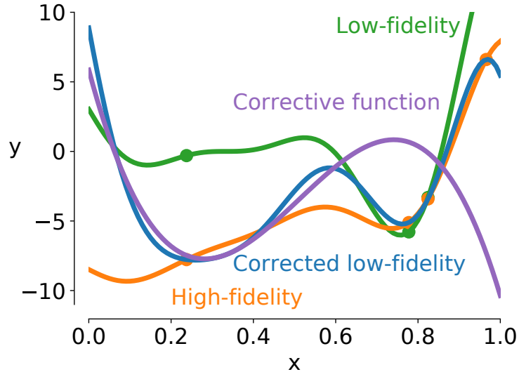
(b) Piecewise-cubic
