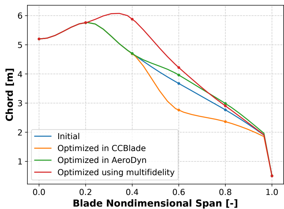
(b) Chord distributions along the blade span
