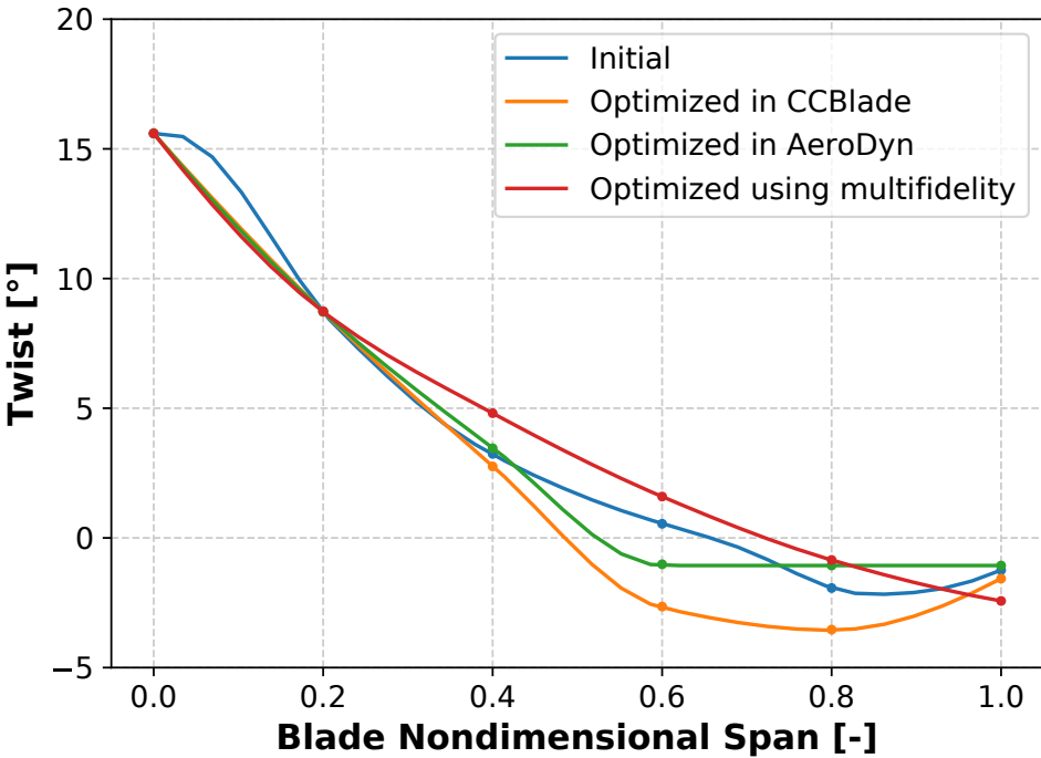
(a) Twist distributions along the blade span
