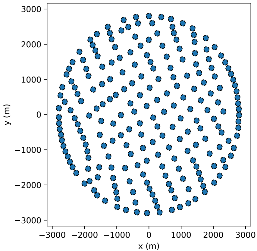
(a) SLSQP, AEP= 1.172e+03 GWh
