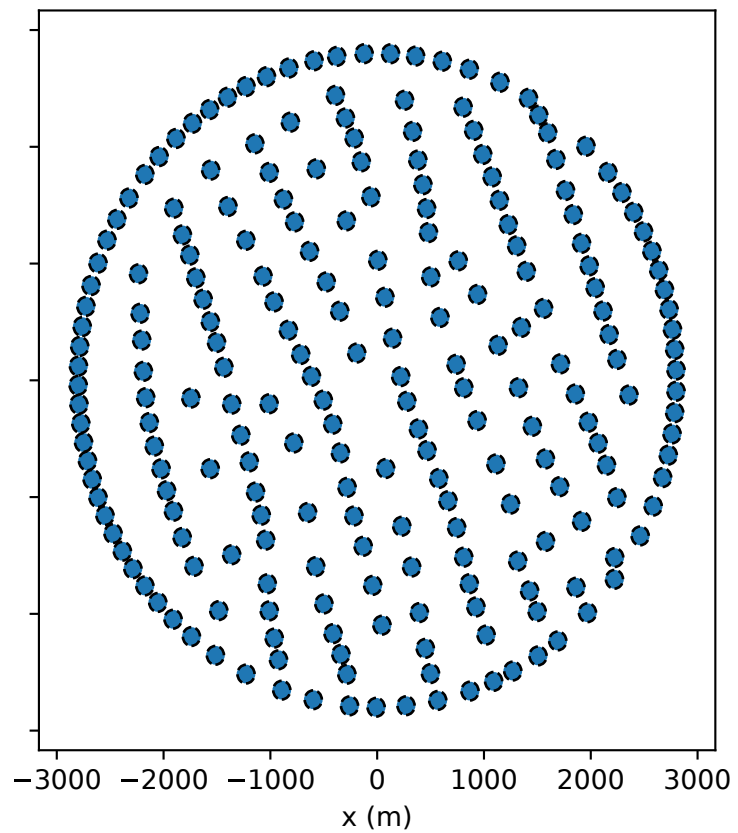
(b) SGD, AEP= 1.180e+03 GWh
