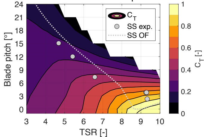
Thrust coefficient - Exp.
