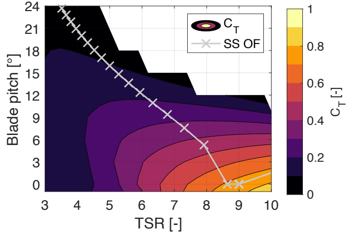
Thrust coefficient - OF
