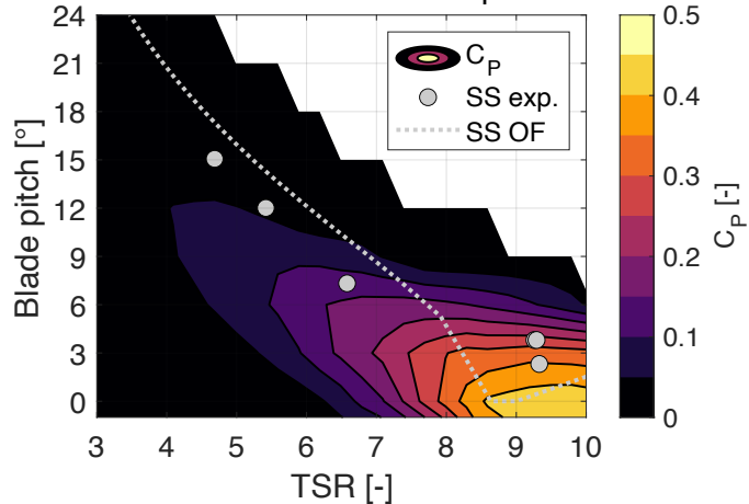
Power coefficient - Exp.
