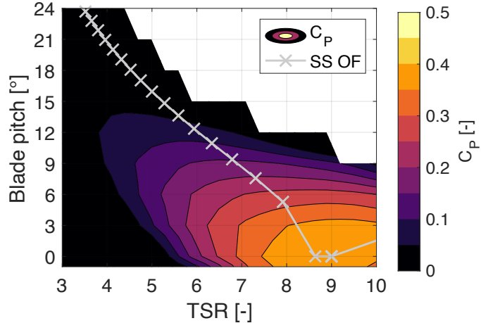
Power coefficient - OF
