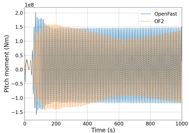
(f) LC 3.1 Pitch moment
