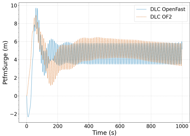
(a) LC 3.1 Surge
