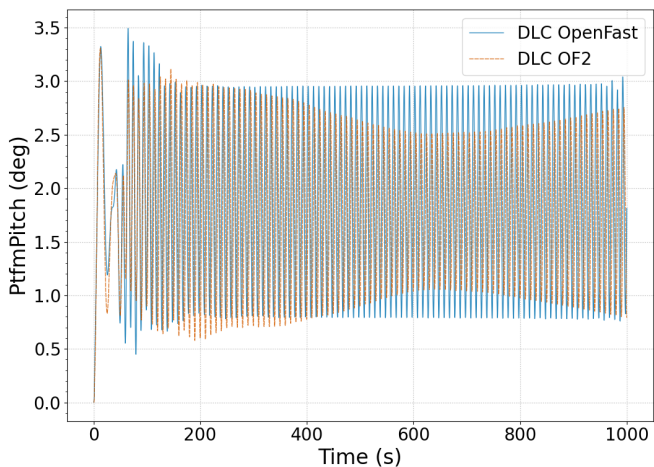
(e) LC 3.1 Pitch
