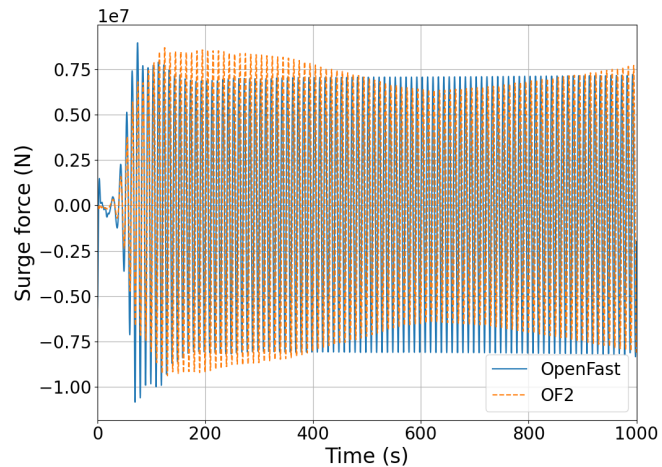
(b) LC 3.1 Surge force
