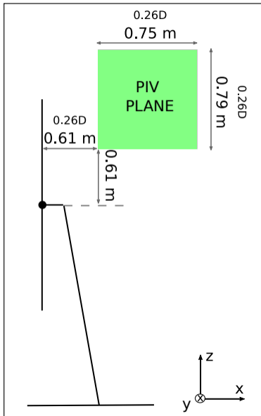
LATERAL VIEW
