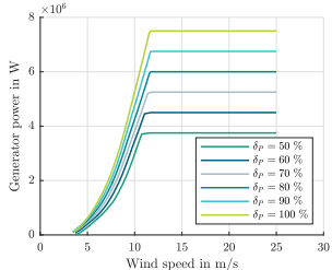
(c) Electrical power over wind speed
