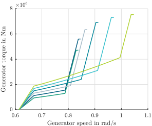
(a) Generator torque over generator speed
