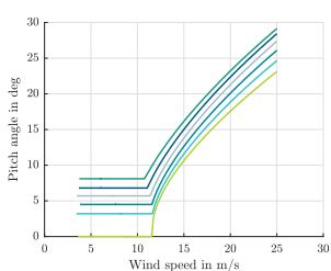
(b) Pitch angle over wind speed
