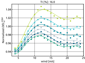
(a) normalized short-term DEL of edgewise BM
