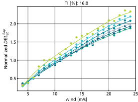
(b) normalized short-term DEL of flapwise BM
