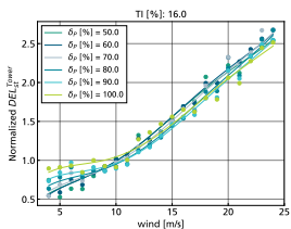
(c) normalized short-term DEL of tower BM
