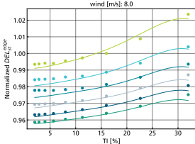
(a) normalized short-term DEL of edgewise BM
