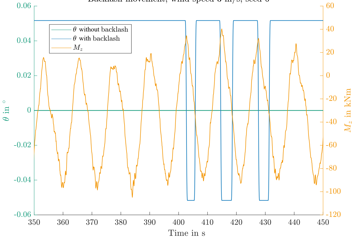
Backlash movement, wind speed 3 m/s, seed 6
