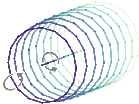
(b) actuator disc with rotation (ADMR)
