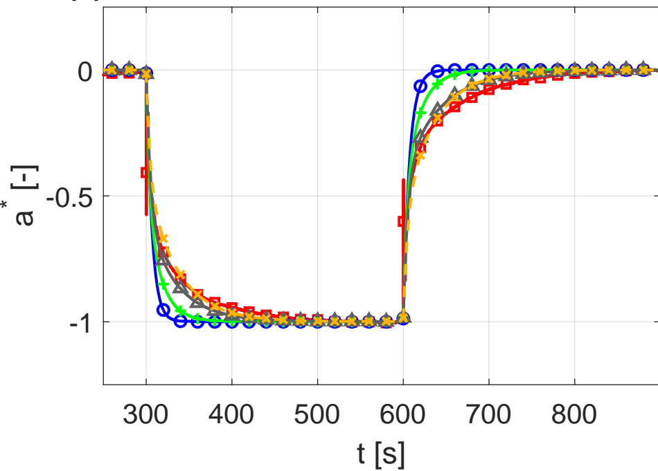
(c) - Normalized Axial induction - r/R = 80\%
