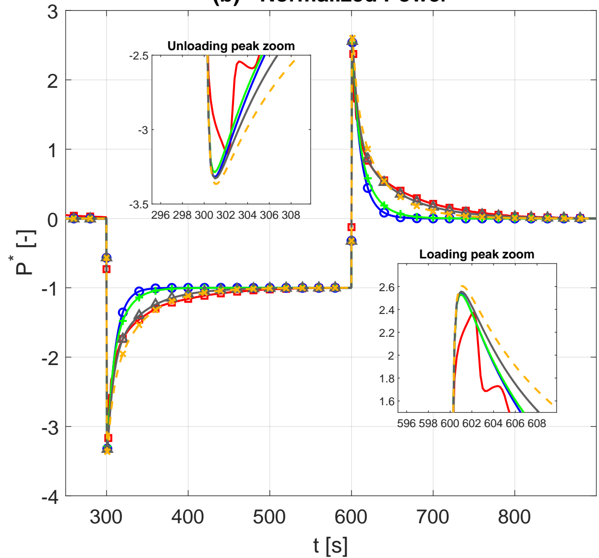
(b) - Normalized Power
