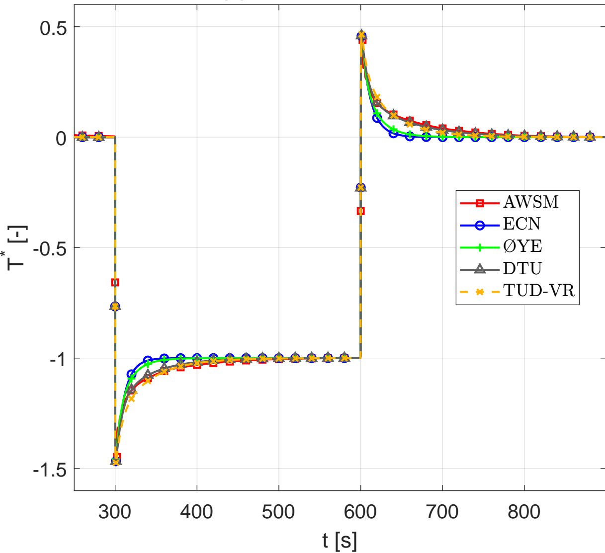
(a) - Normalized Thrust
