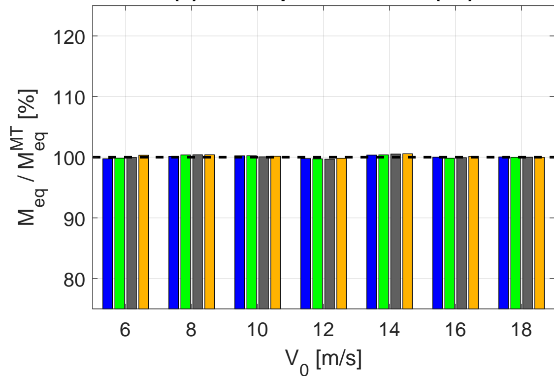
(b) root in-plane moment (B1)
