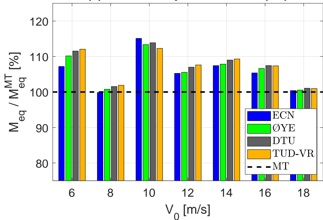
(a) root out-of-plane moment (B1)
