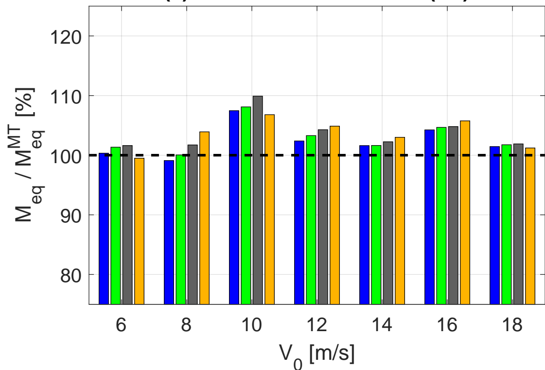
(c) root torsional moment (B1)
