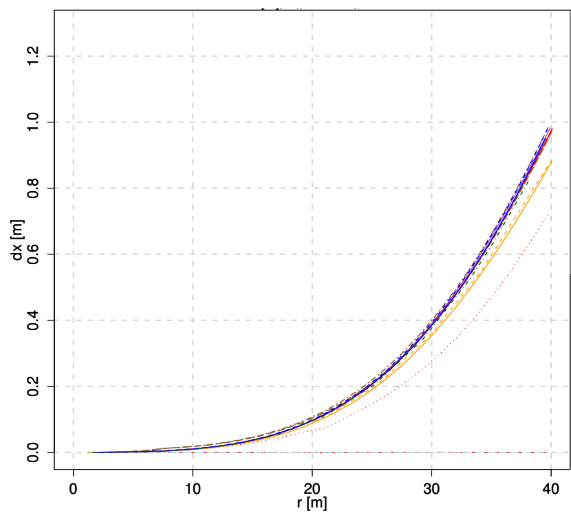
(e) Flapwise deformation dx
