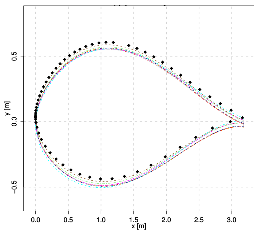
(a) Sectional geometry at r=13.12 m
