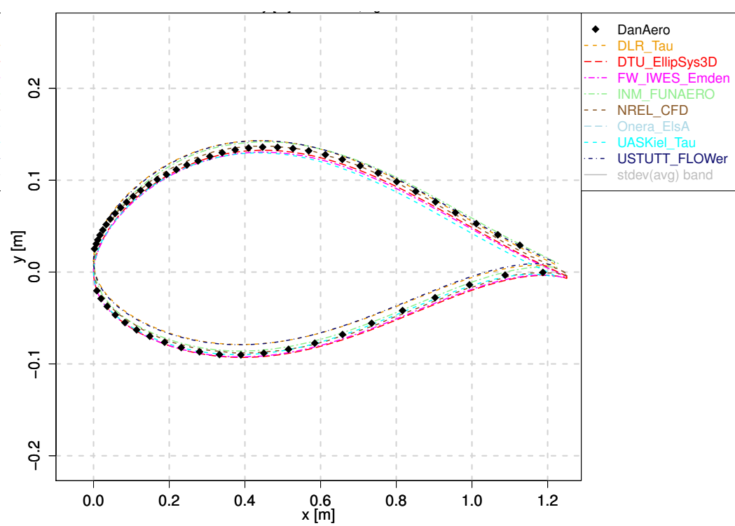
(b) Sectional geometry at r=36.78 m
