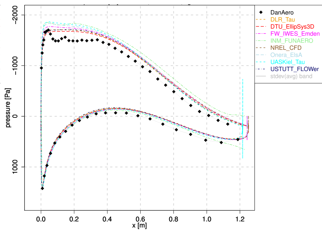
(f) Pressure at r=36.78 m
