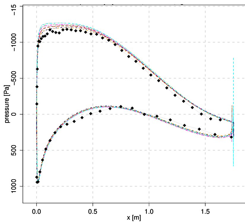
(e) Pressure at r=30.20 m
