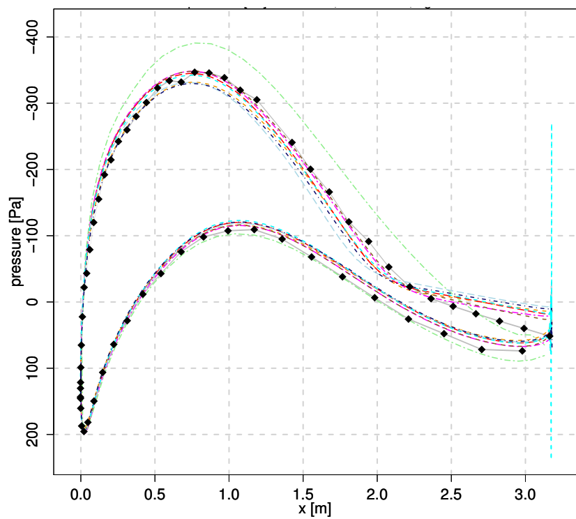
(c) Pressure at r=13.12 m
