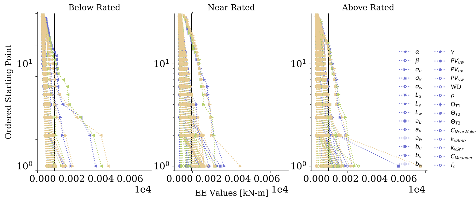
(b) Fatigue loads
