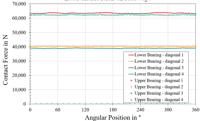
Load distribution on raceways
