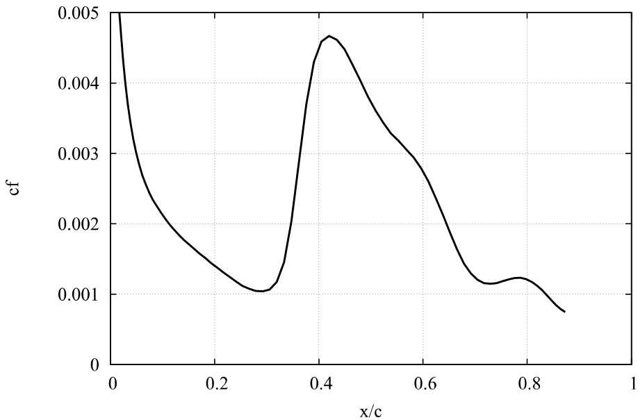
Friction coefficient at R=35 , Re=2.9M , N=5 and AOA=2^\circ
