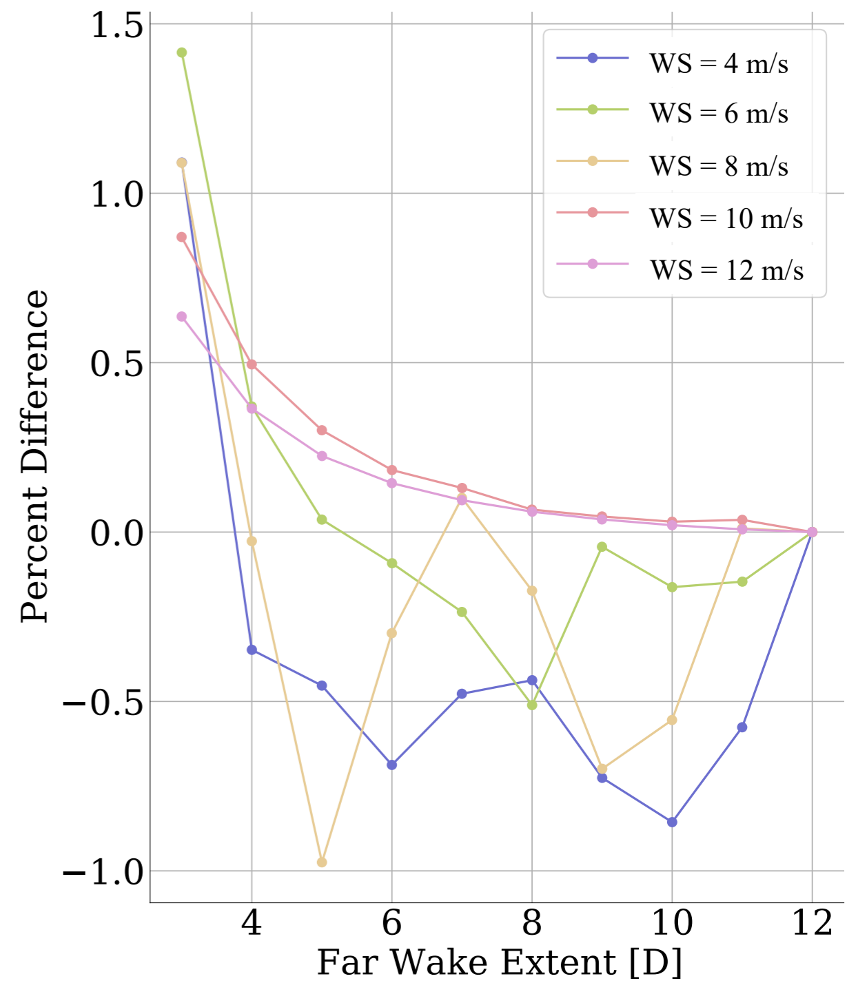
(c) Far wake extent convergence
