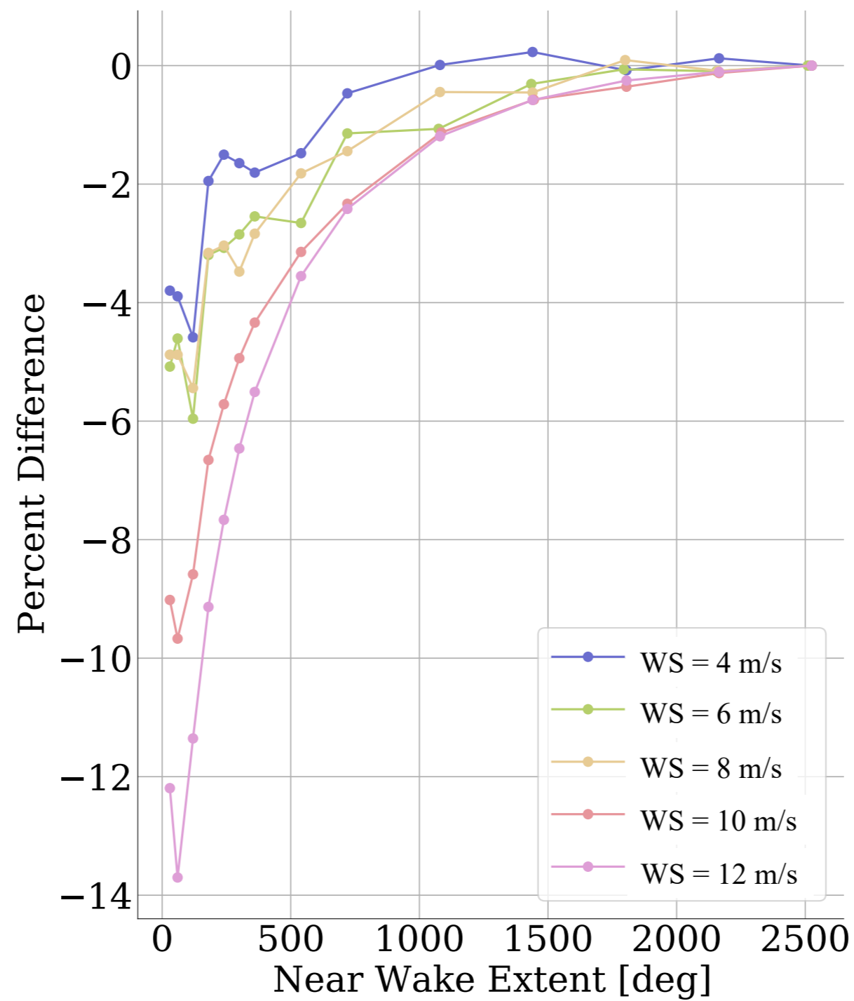
(b) Near wake extent convergence
