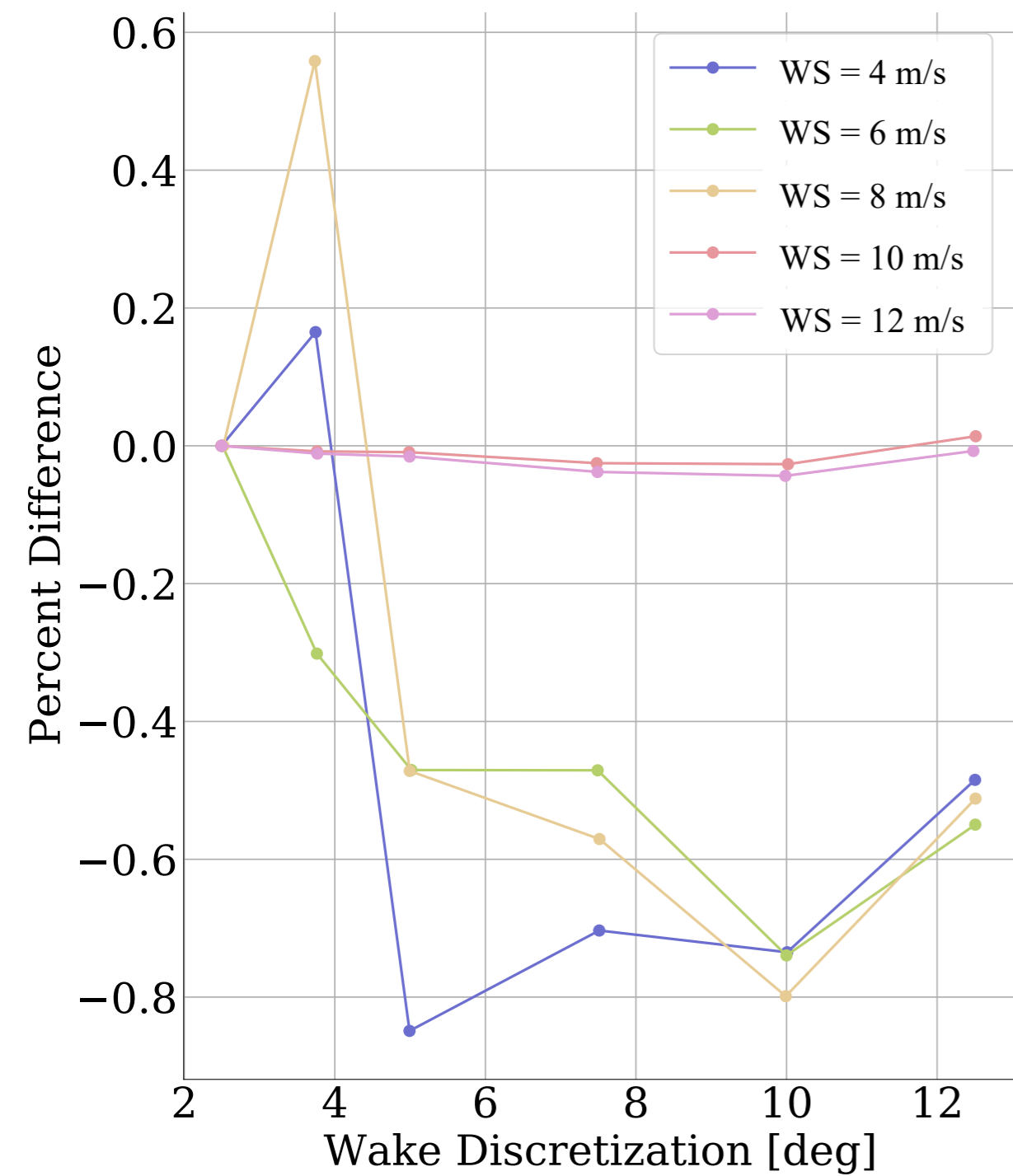
(a) Wake discretization convergence
