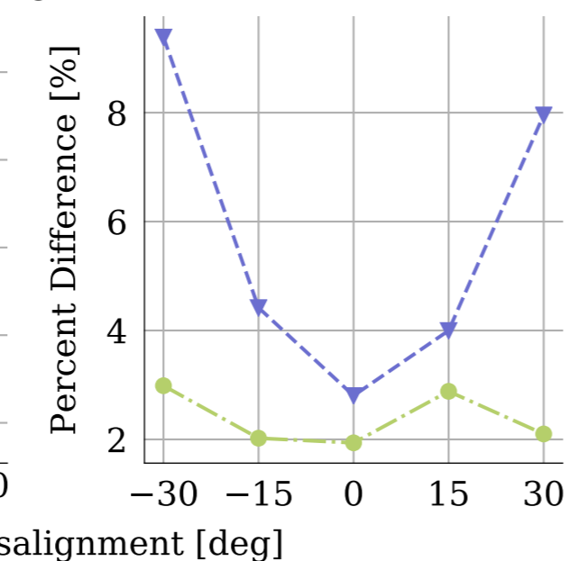
(g) Fore/aft tower-base bending moment
