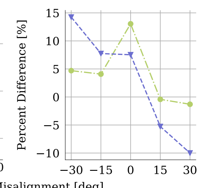
(f) Side/side tower-base bending moment
