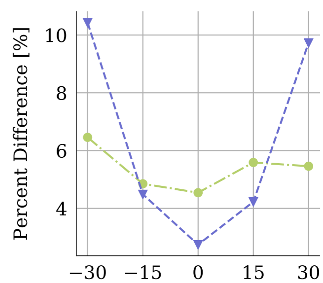
(b) Out-of-plane blade deflection
