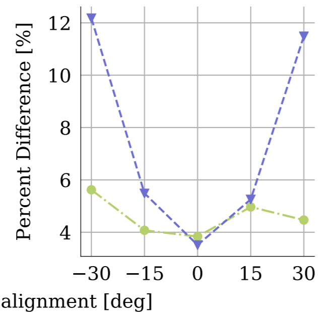
(c) Out-of-plane blade-root bending moment
