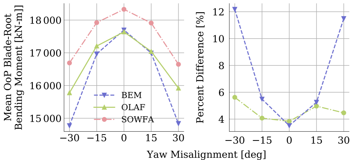
(c) Out-of-plane blade-root bending moment
