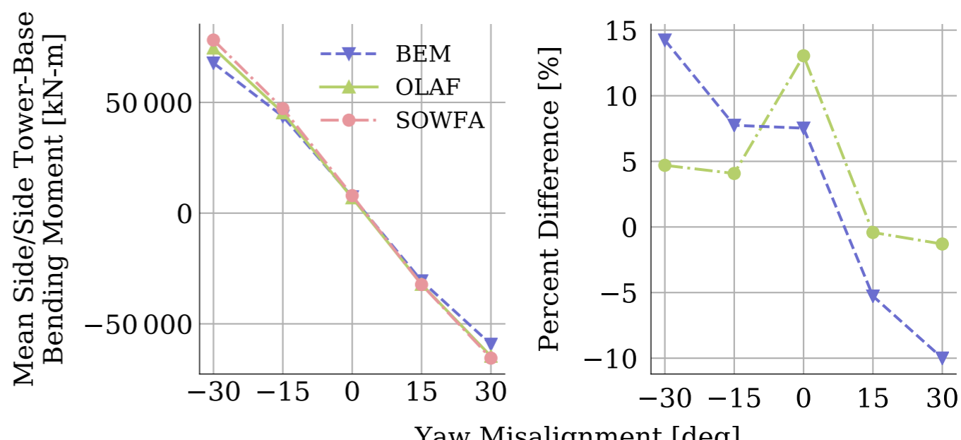
(f) Side/side tower-base bending moment
