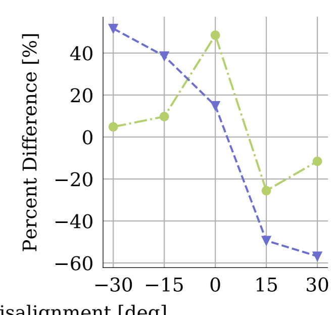
(h) Tower-base yaw moment
