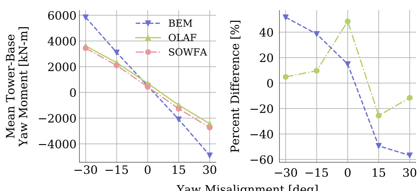
(h) Tower-base yaw moment
