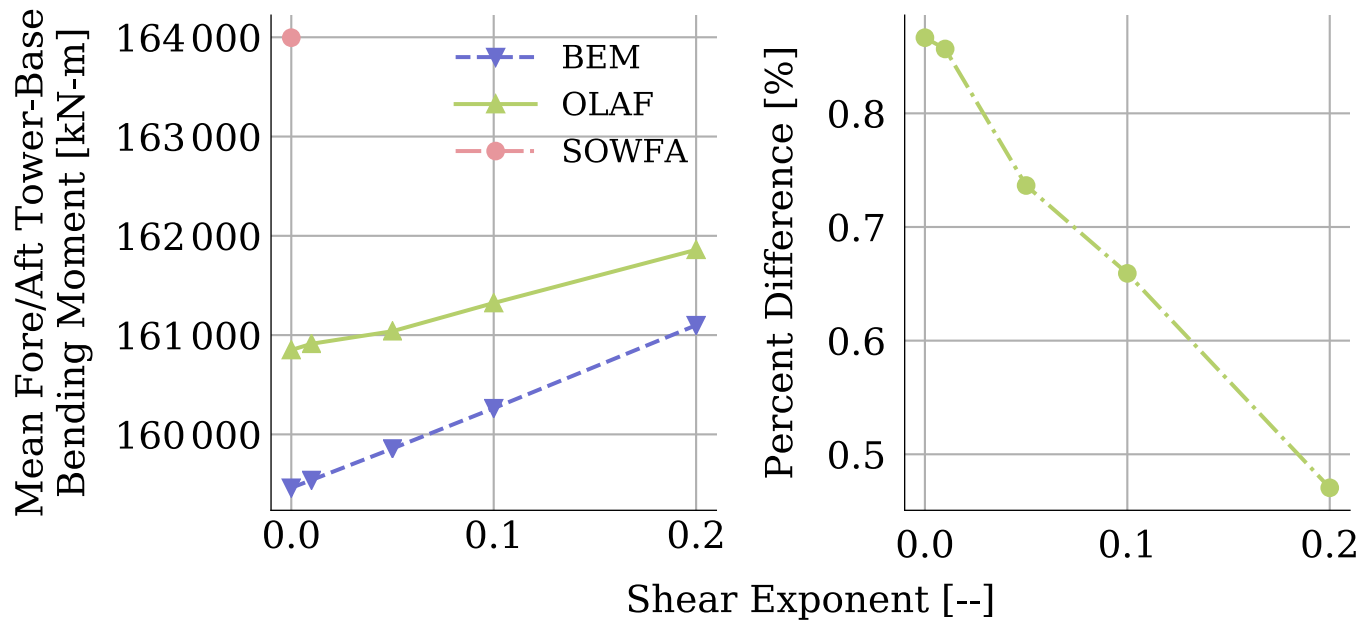
(c) Fore/aft tower-base bending moment
