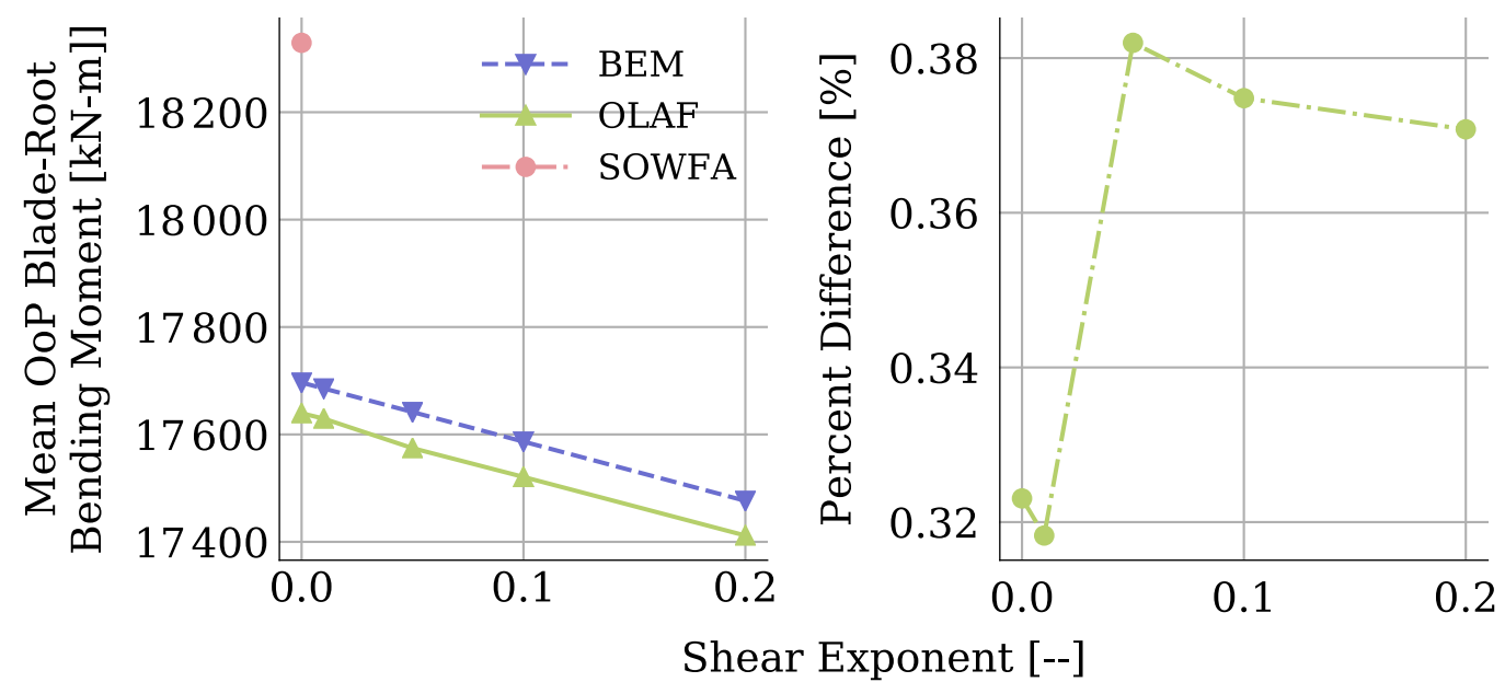
(b) Out-of-plane blade-root bending moment
