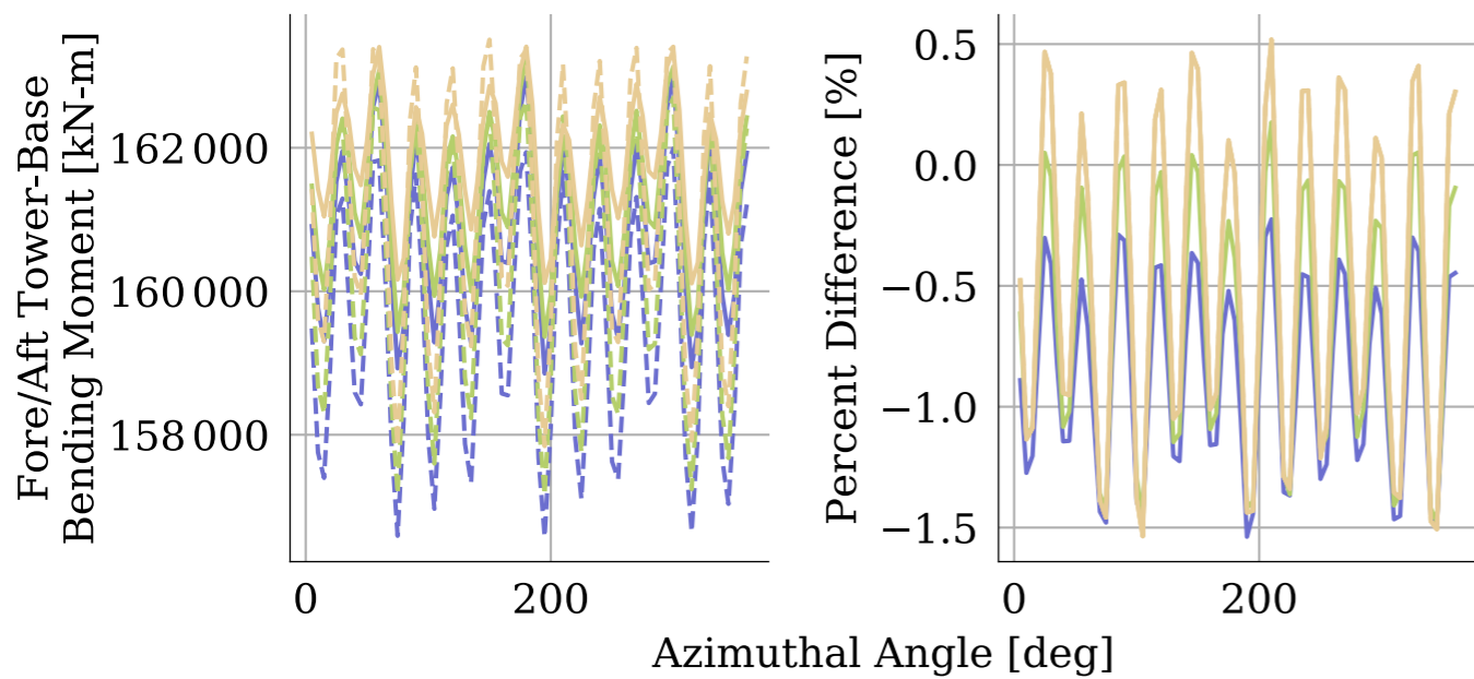
(c) Fore/aft tower-base bending moment
