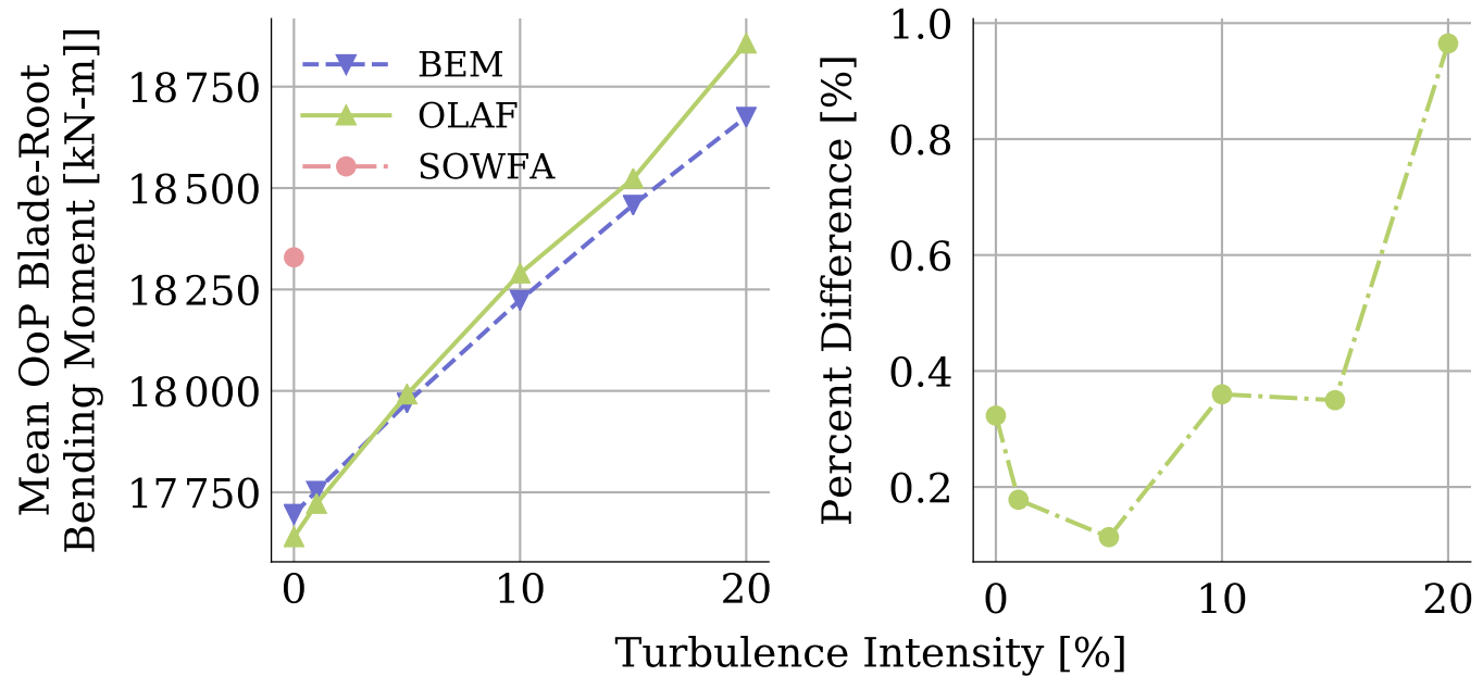
(b) Mean out-of-plane blade-root bending moment
