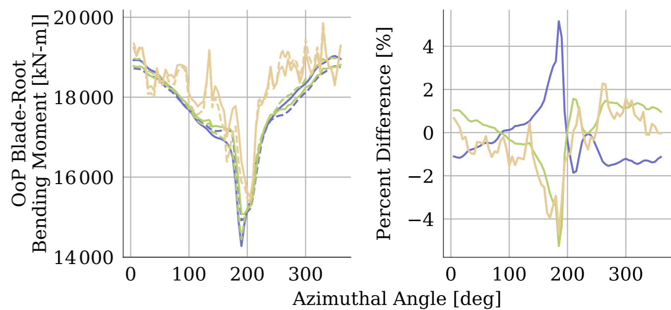
(b) Out-of-plane blade-root bending
