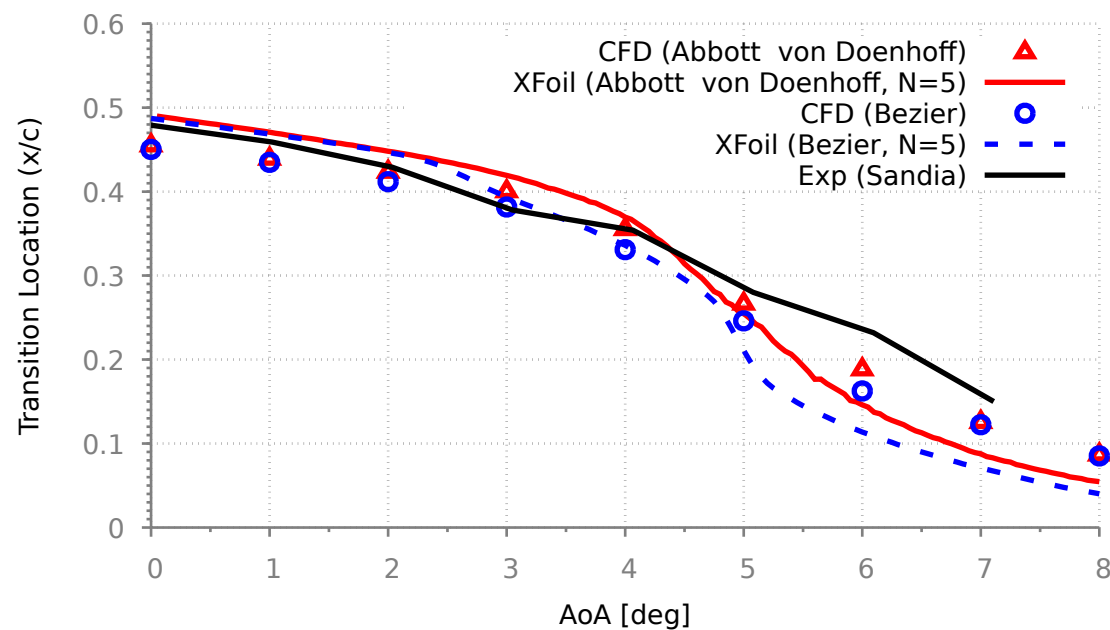
Suction side transition location Airfoil: NACA 63-418, Re = 3.2E6 Solver: OpenFOAM, RASModel: RANS kOmegaSSTLM, Ti: 0.8\%
