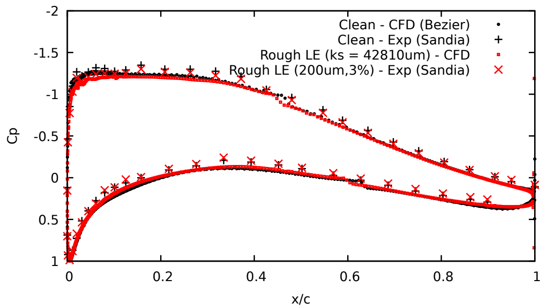
Airfoil: NACA 63-418, Re = 3.2E6 Solver: OpenFOAM, RASModel: RANS kOmegaSSTLMkvAr, Ti: 0.8 % AoA = 8deg
