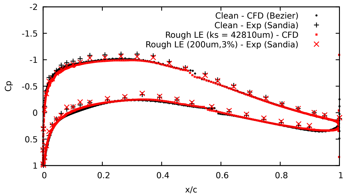
Airfoil: NACA 63-418, Re = 3.2E6 Solver: OpenFOAM, RASModel: RANS kOmegaSSTLMkvAr, Ti: 0.8 % AoA = 6deg
