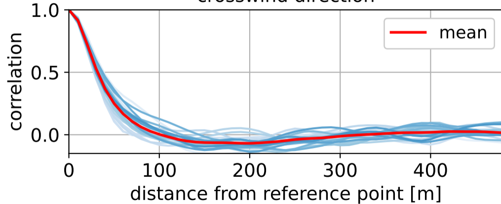
crosswind direction
