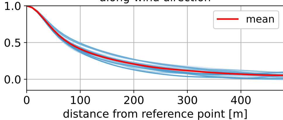
along-wind direction
