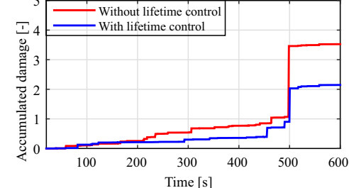
(c) Blade damage accumulation
