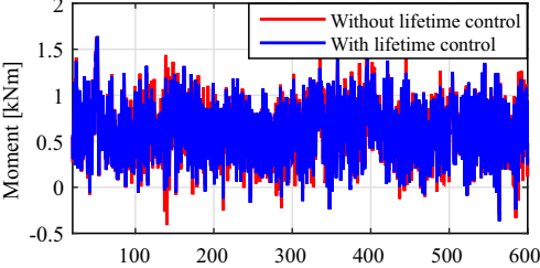
(b) Blade F-W bending moment
