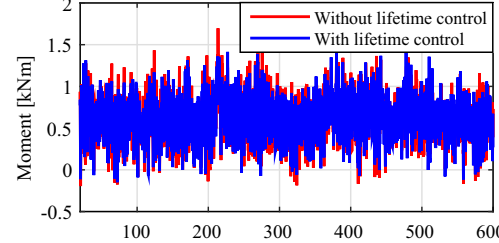
(b) Blade F-W bending moment
