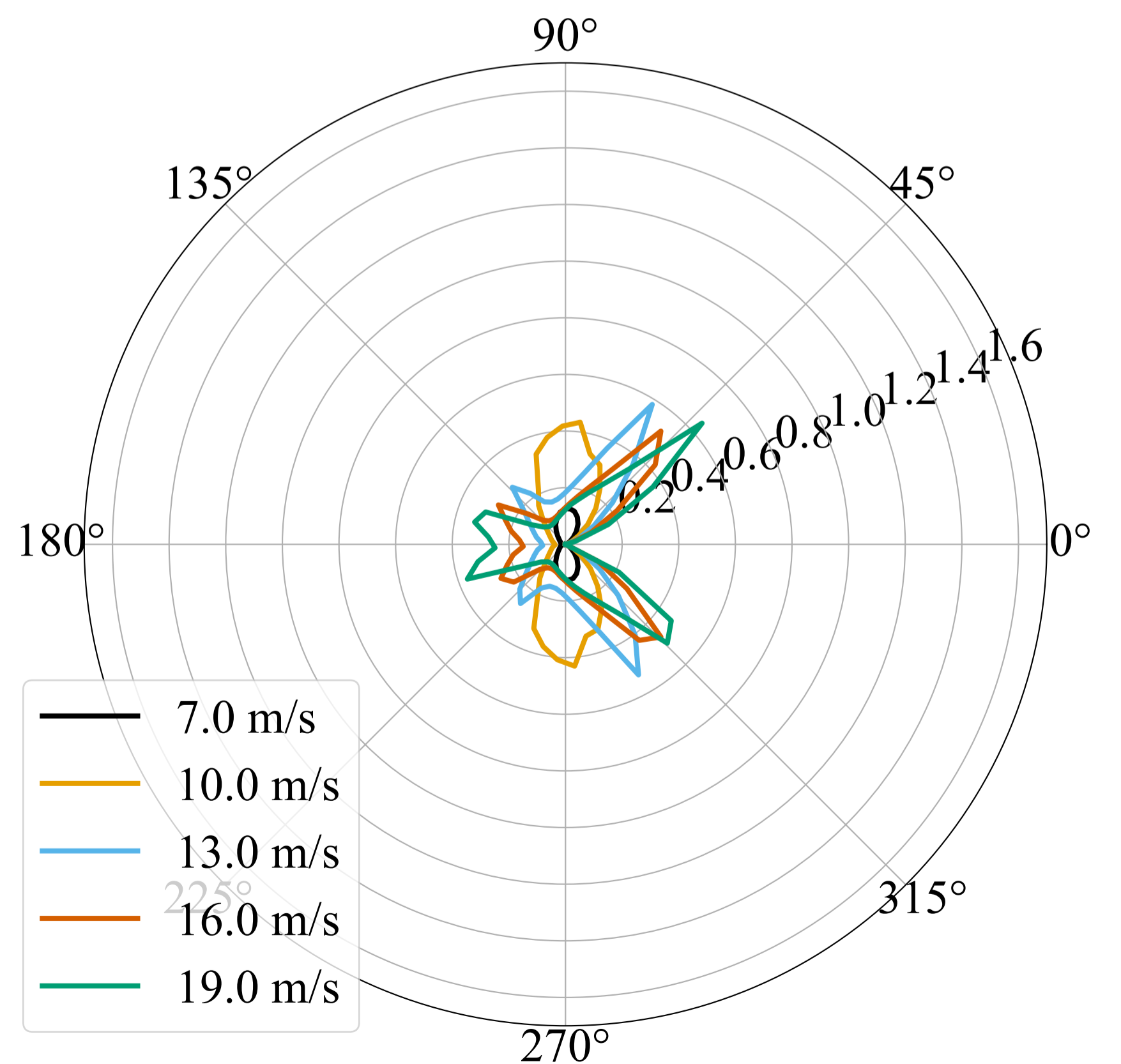
(c) Flettner rotor consumed power ( P_p , MW)
