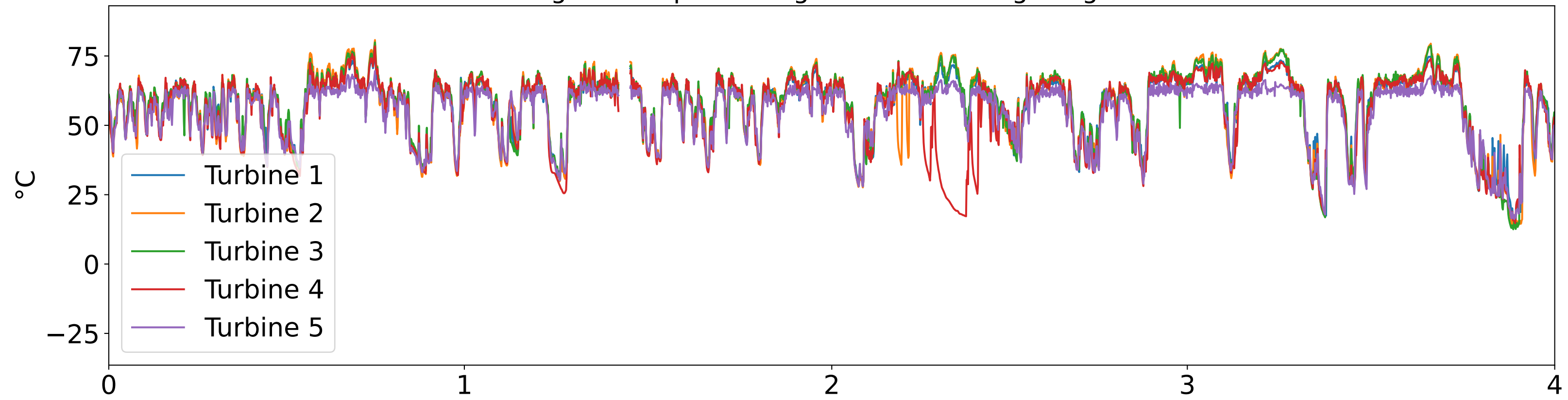
Common component temperature generator bearing 1 (fleet median)
