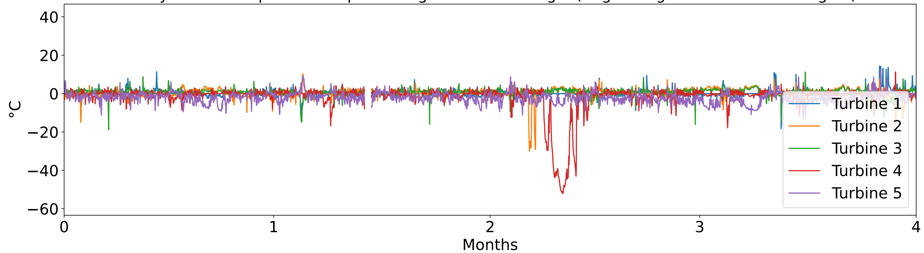
Idiosyncratic component temperature generator bearing 1 (original signal - fleet median signal)
