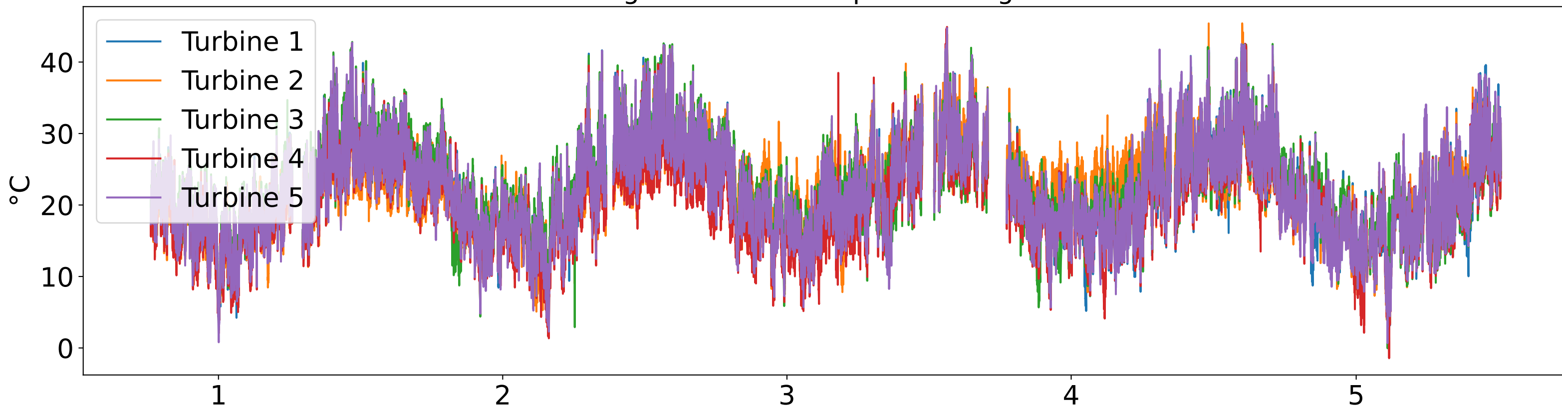
Common component nacelle temperature (fleet median)
