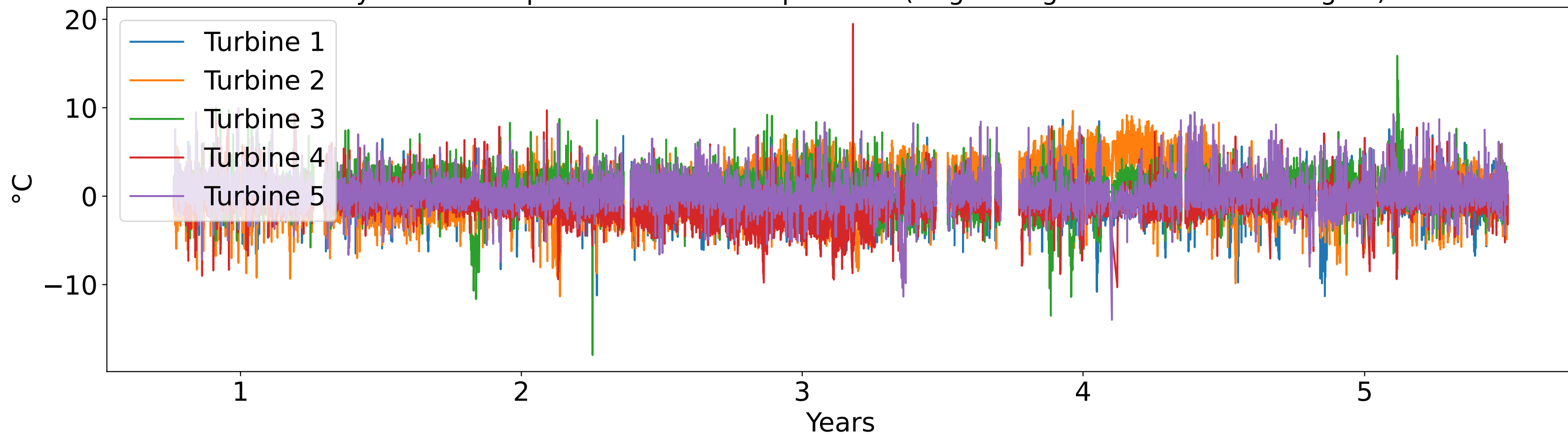
Idiosyncratic component nacelle temperature (original signal - fleet median signal)
