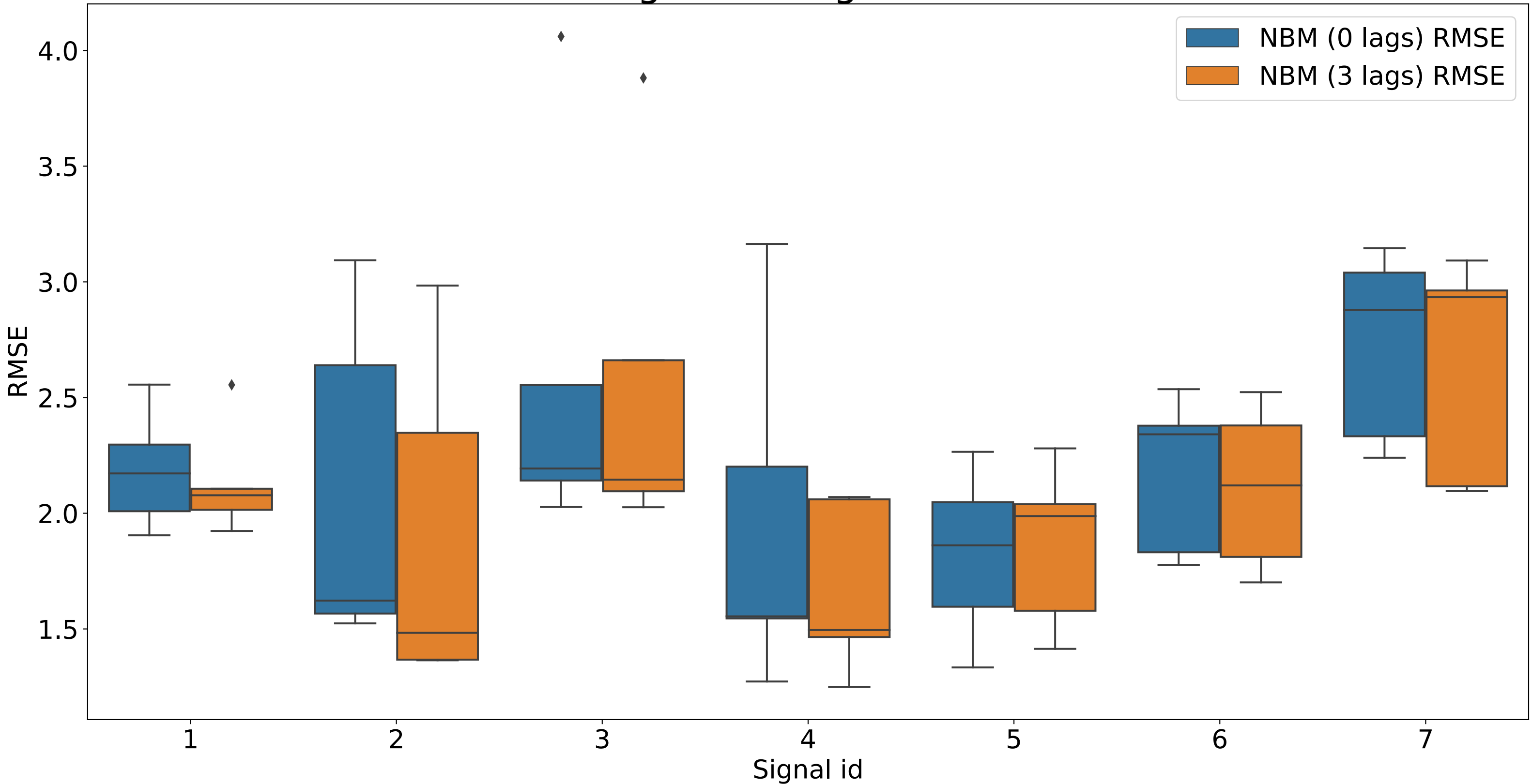
RMSE of no lags vs. 3 lags for wind farms 1-5
