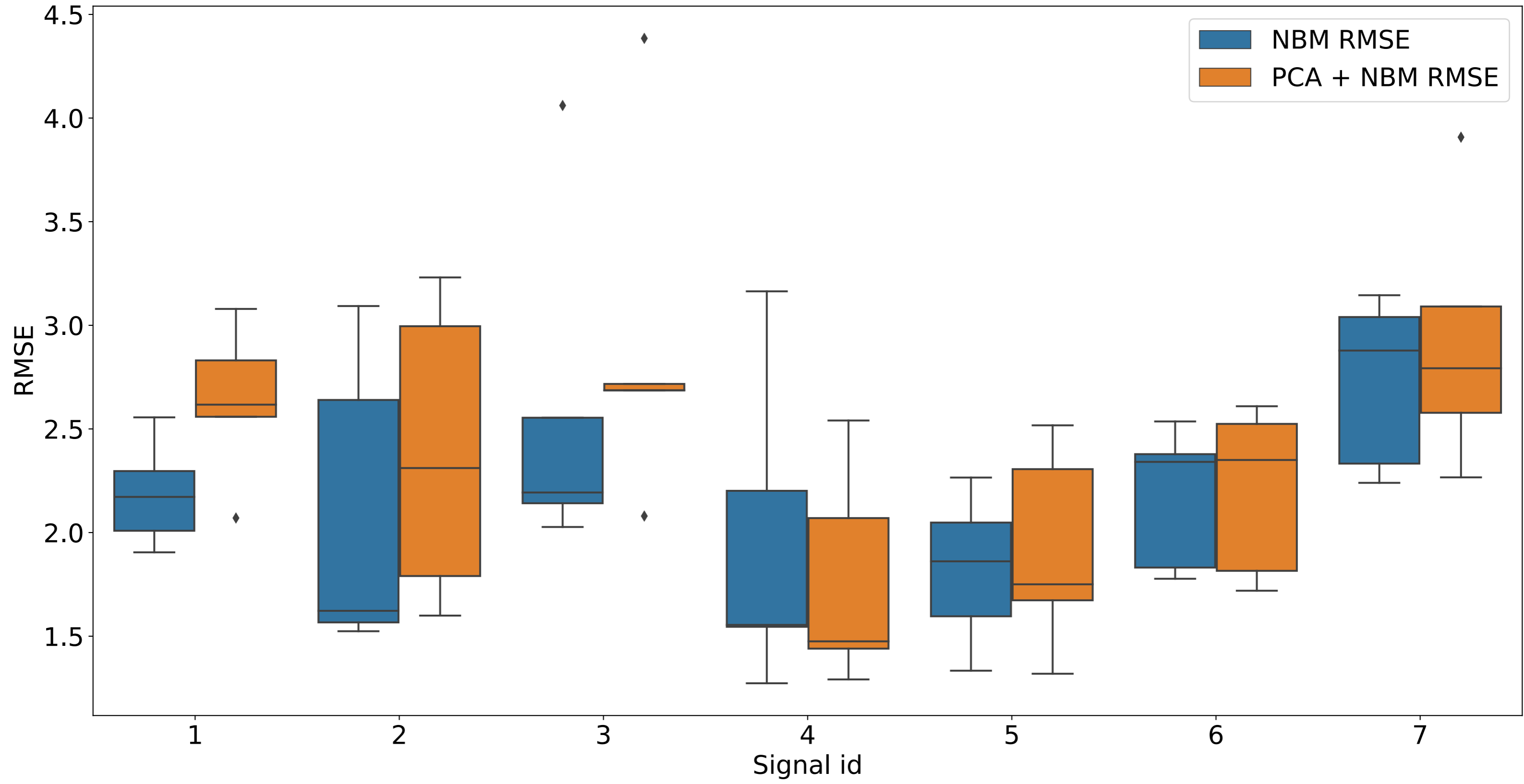
RMSE for PCA vs. no PCA for wind farms 1-5
