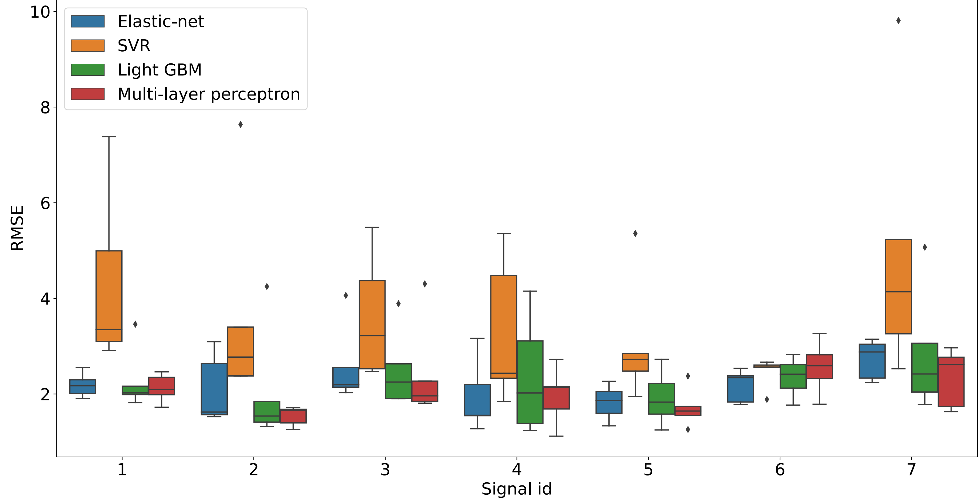
RMSE for elastic net vs. SVR vs. light GBM vs. MLP for wind farms 1-5
