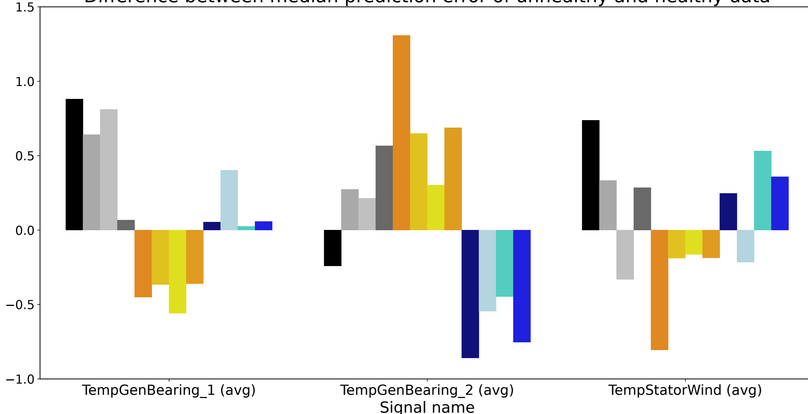
Difference between median prediction error of unhealthy and healthy data
