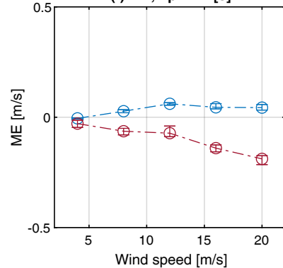
(f) ME, T_p = 11 [s]
