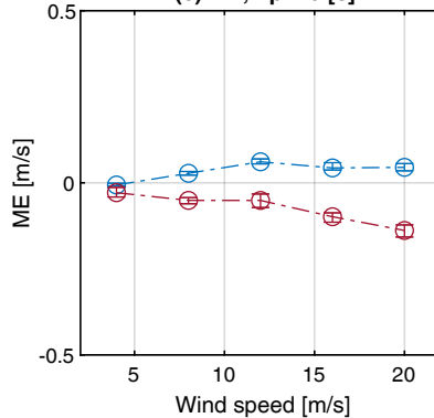
(e) ME, T_p = 9 [s]
