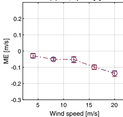
(b) ME, T_p = 9 [s]
