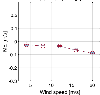
(a) ME, T_p = 6 [s]
