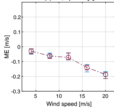
(c) ME, T_p = 11 [s]
