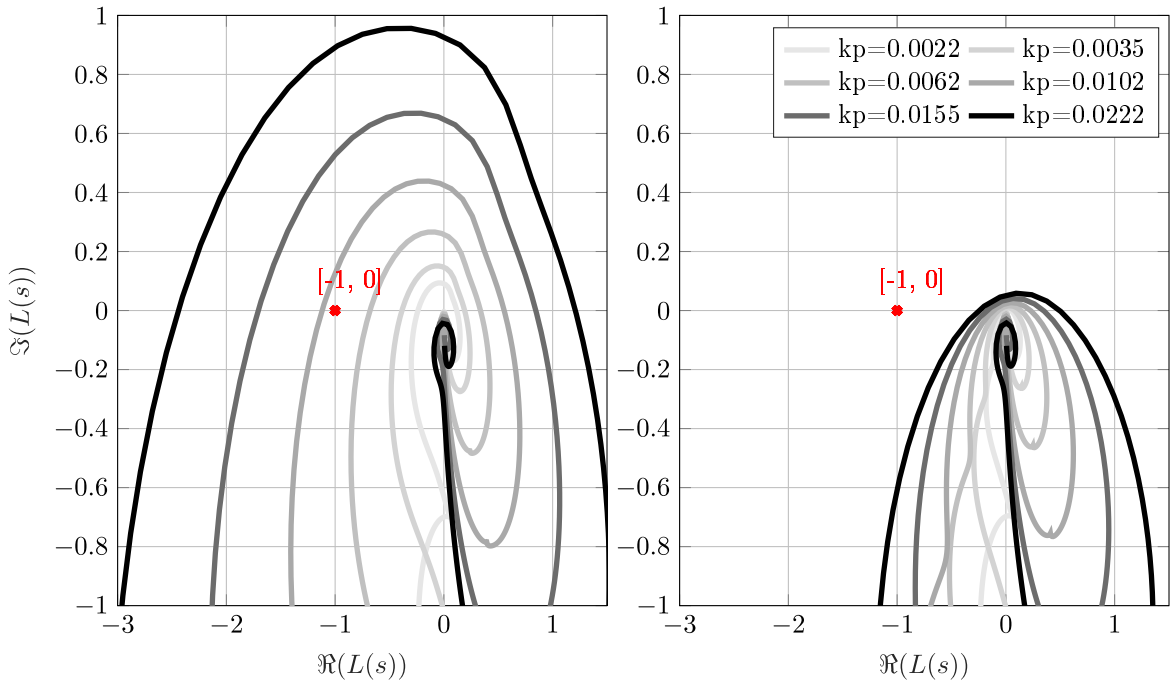
Nyquist plot of open-loop system L(s) : reference (left); TLMCD activated (right)
