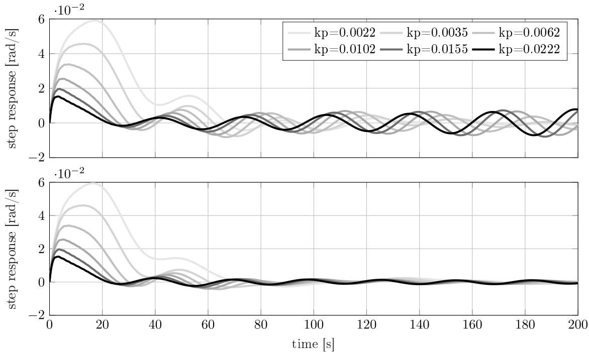
Step response with variable k_p : reference (above); TLMCD activated (below)
