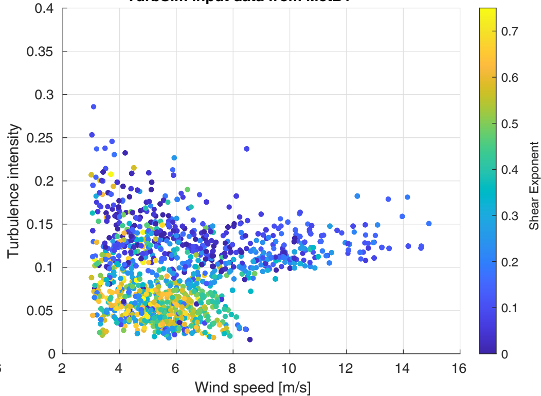
TurbSim input data from MetB1
