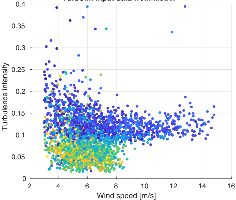
TurbSim input data from MetA1
