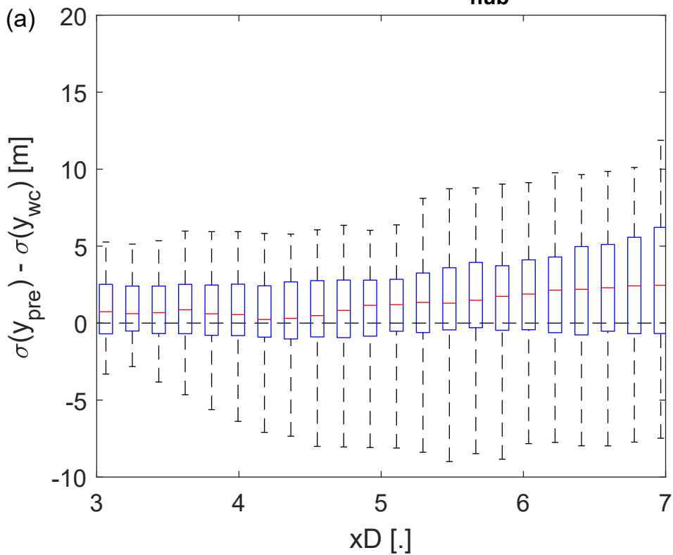
Prediction with u_{\text{hub}}
