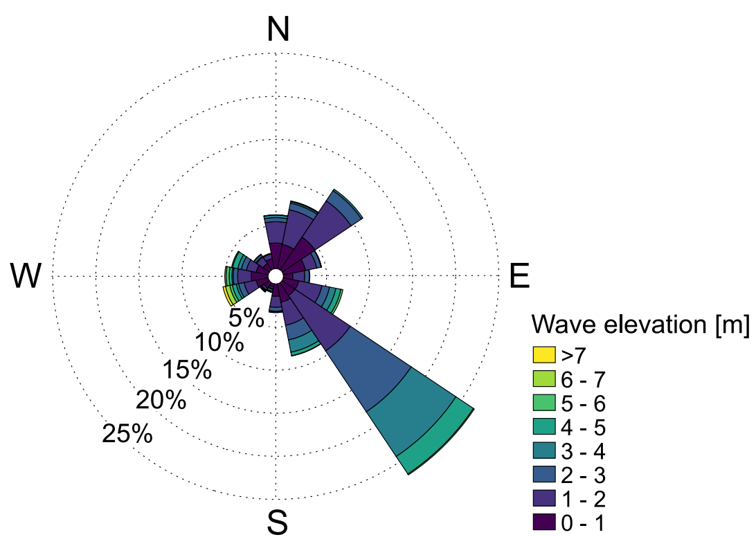
Wave rose
