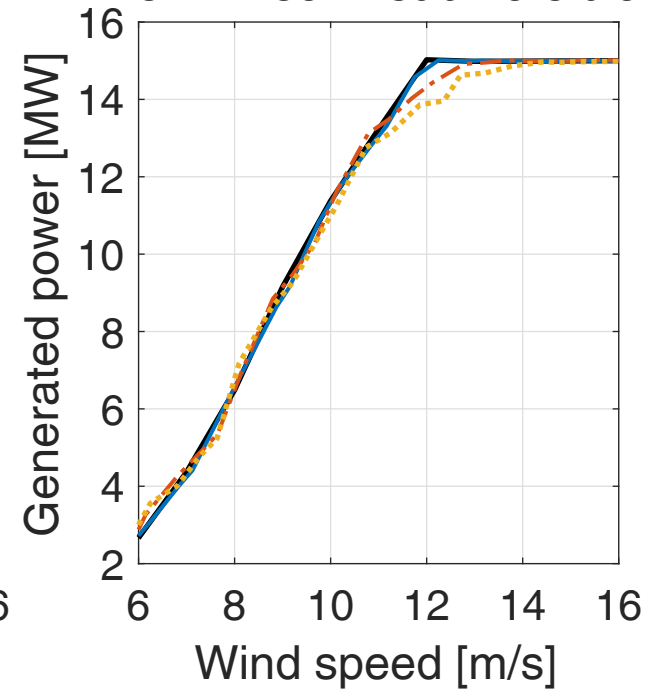
15 MW semi-submersible
