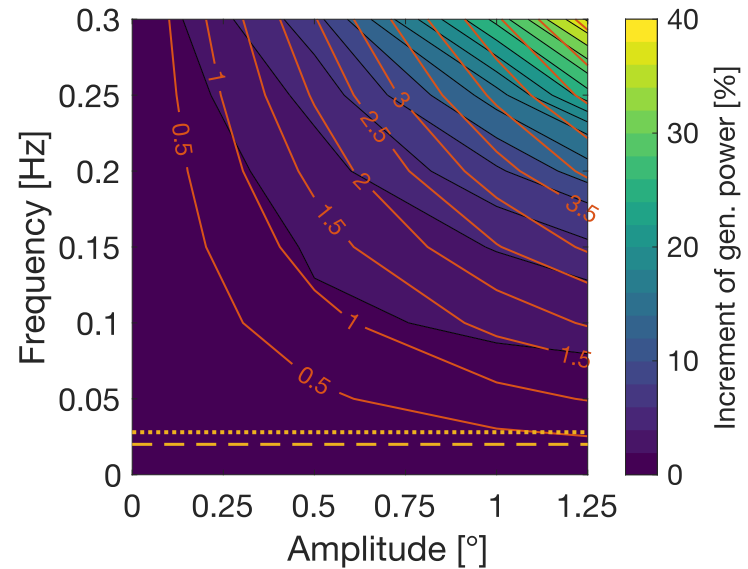
15 MW – Pitch
