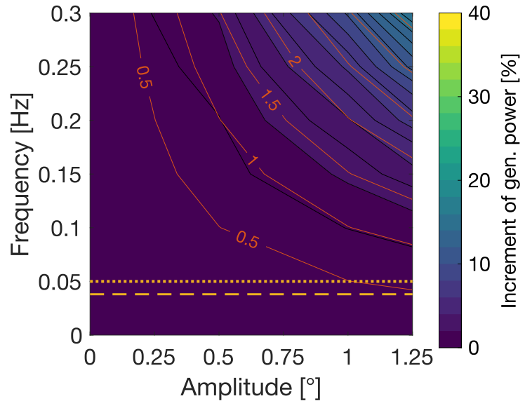
5 MW – Pitch
