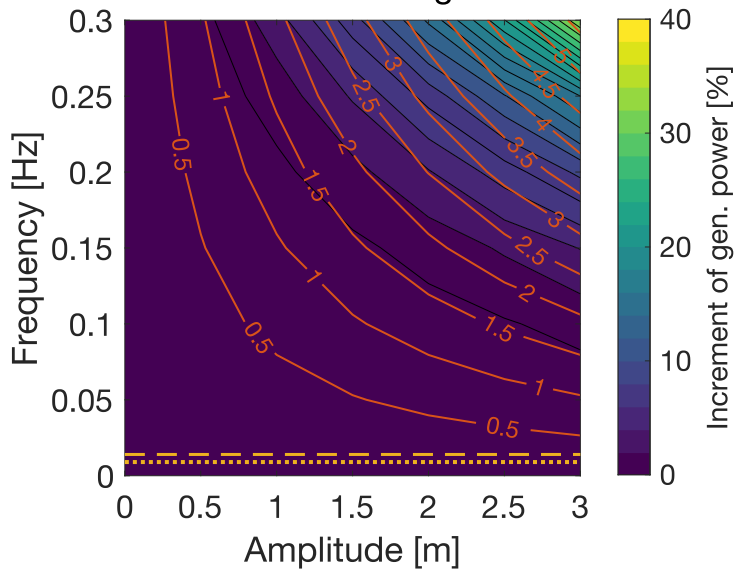
15 MW – Surge
