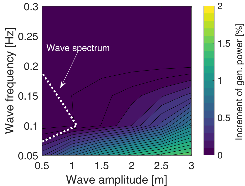
5 MW semi-submersible
