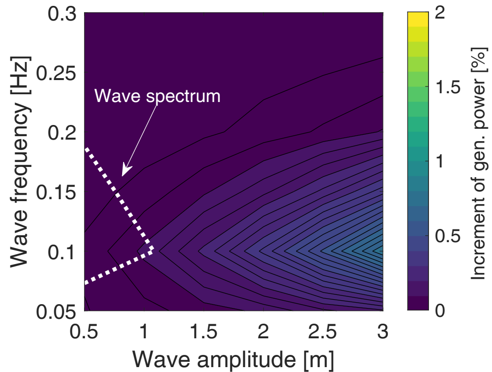
15 MW semi-submersible
