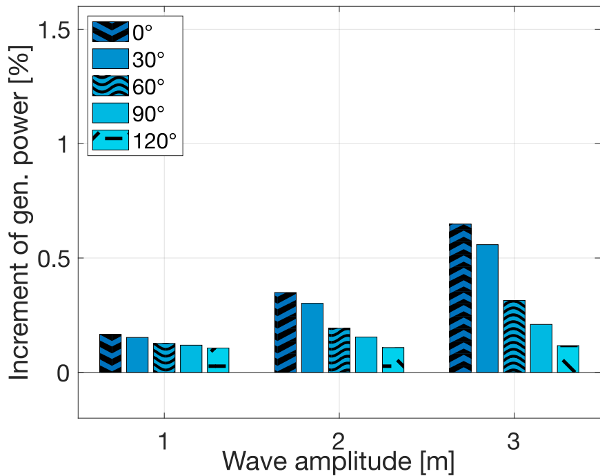
5 MW semi-submersible
