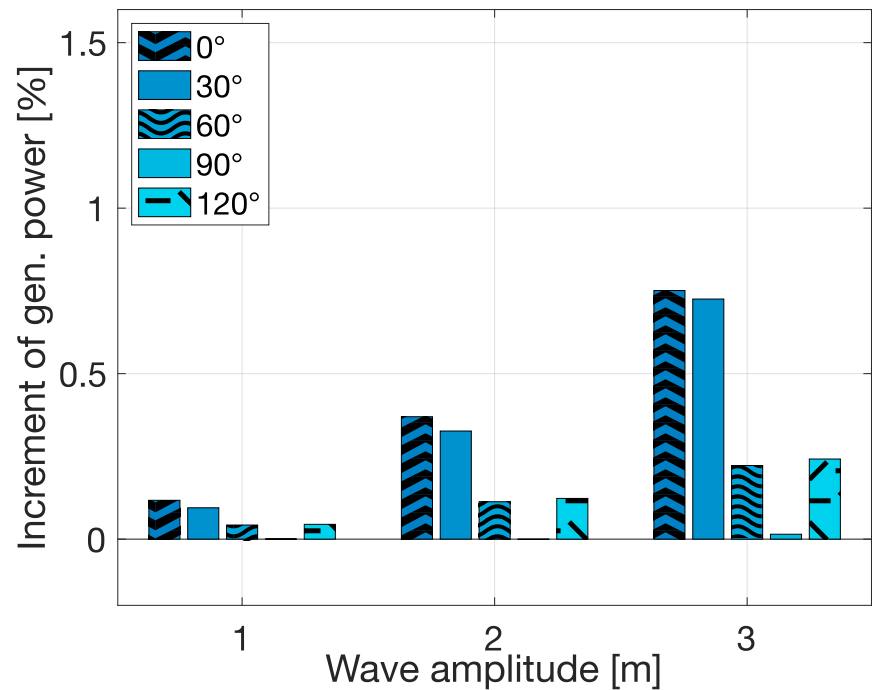
15 MW semi-submersible
