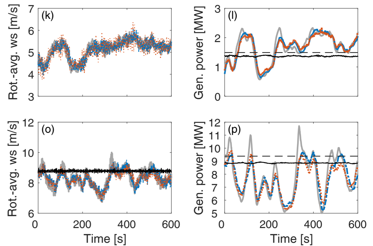
15 MW semi-submersible
