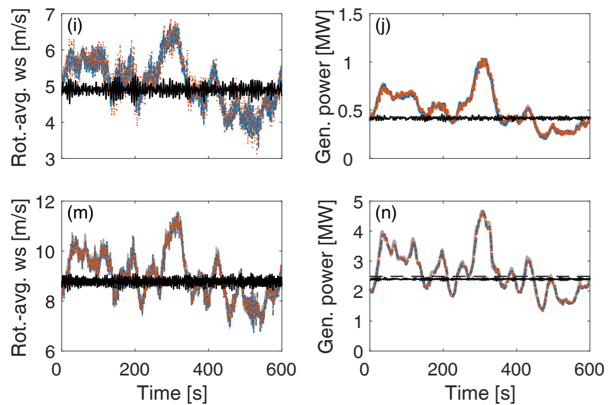
5 MW semi-submersible
