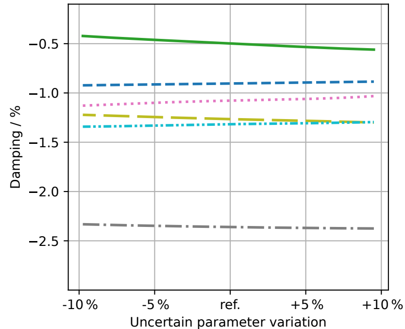
Edgewise Stiffness
